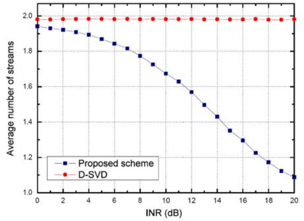
Fig. 3. Average number of streams vs. INR for L = 2 , N_t = 2 , N_r = 2 , and \text{SNR} = 20\text{dB} .
