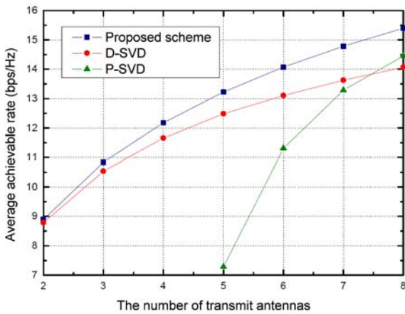
Fig. 5. Average achievable rate vs. N_t for L = 3 , N_r = 2 , \text{SNR} = 20\text{dB} , and \text{INR} = 0\text{dB} .
