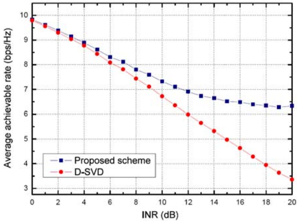
Fig. 2. Average achievable rate vs. INR for L = 2 , N_t = 2 , N_r = 2 , and \text{SNR} = 20\text{dB} .
