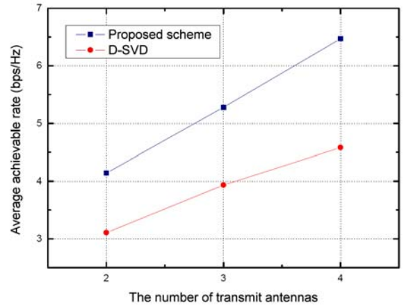
Fig. 6. Average achievable rate vs. N_t for 7 hexagon cells with N_r = 2 .
