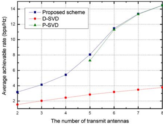
Fig. 4. Average achievable rate vs. N_t for L = 3 , N_r = 2 , \text{SNR} = 20\text{dB} , and \text{INR} = 20\text{dB} .
