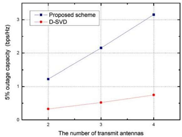
Fig. 7. 5% outage capacity vs. N_t for 7 hexagon cells with N_r = 2 .
