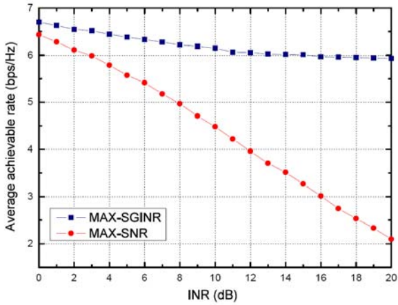
Fig. 1. Average achievable rate vs. INR for L = 2 , N_t = 2 , N_r = 1 , and \text{SNR} = 20\text{dB} .
